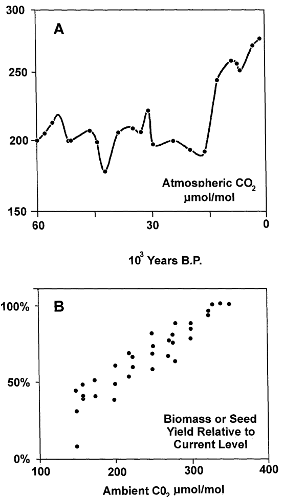
Figure 3. Panel A shows the curve of atmospheric \text{CO}_2 as estimated from gas bubbles trapped in Antarctic glacial ice. Data from Barnola et al. (1987). Panel B summarizes responses of several plant species to experimental atmospheres containing various levels of \text{CO}_2 . Based on data summarized by Sage (1995).
