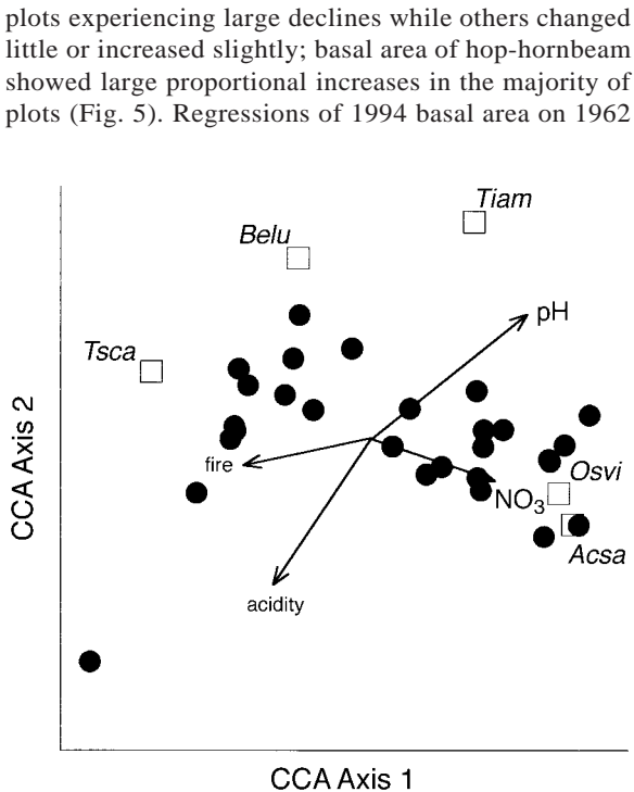
FIG. 3. Canonical correspondence analysis (CCA) biplot of 1994 data, showing first and second axes. Sample and species arrangements are indicated as in Fig. 2. Vectors indicate the strength and sign of correlation of indicated environmental variables with ordination axes (e.g., soil acidity is negatively correlated with both axis 1 and 2). “Fire” is a qualitative variable, coded 1 for plots that burned circa 1825, 0 for unburned plots.
