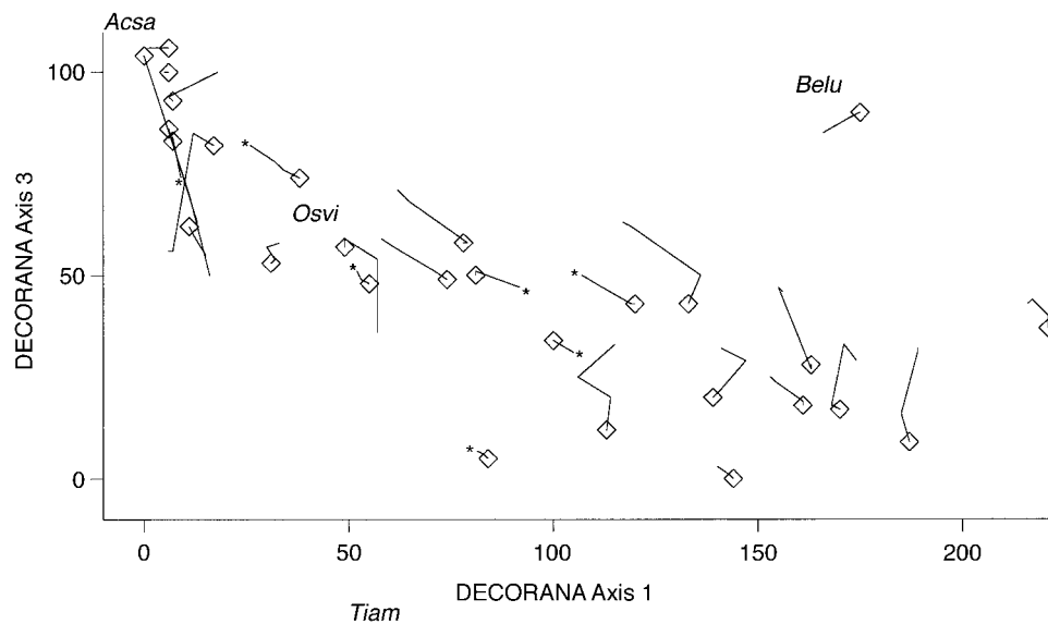
FIG. 4. Plot trajectories in DECORANA ordination space. Ordination includes all measurements of all plots. Lines connect ordinated positions for each plot for successive dates in the temporal sequence. Diamonds represent the most recent (1994) measurement. "New" plots, established in 1978, are indicated by asterisks at the origin of the trajectory. Species centers are as in Fig. 2; Tilia americana is centered below the displayed range on Axis 3.
