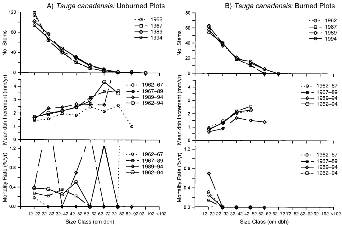
FIG. 8. Demographic patterns for Tsuga canadensis by plot groups. Data are presented as for Fig. 6. Burned plots (plot group IV) are presented separately from remaining plots (plot groups II and III).
